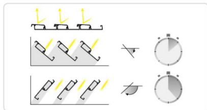
STANDARD SUN PROTECTION LOUVRES: Keeps light out when opening (ideal for frequent use in summer)
